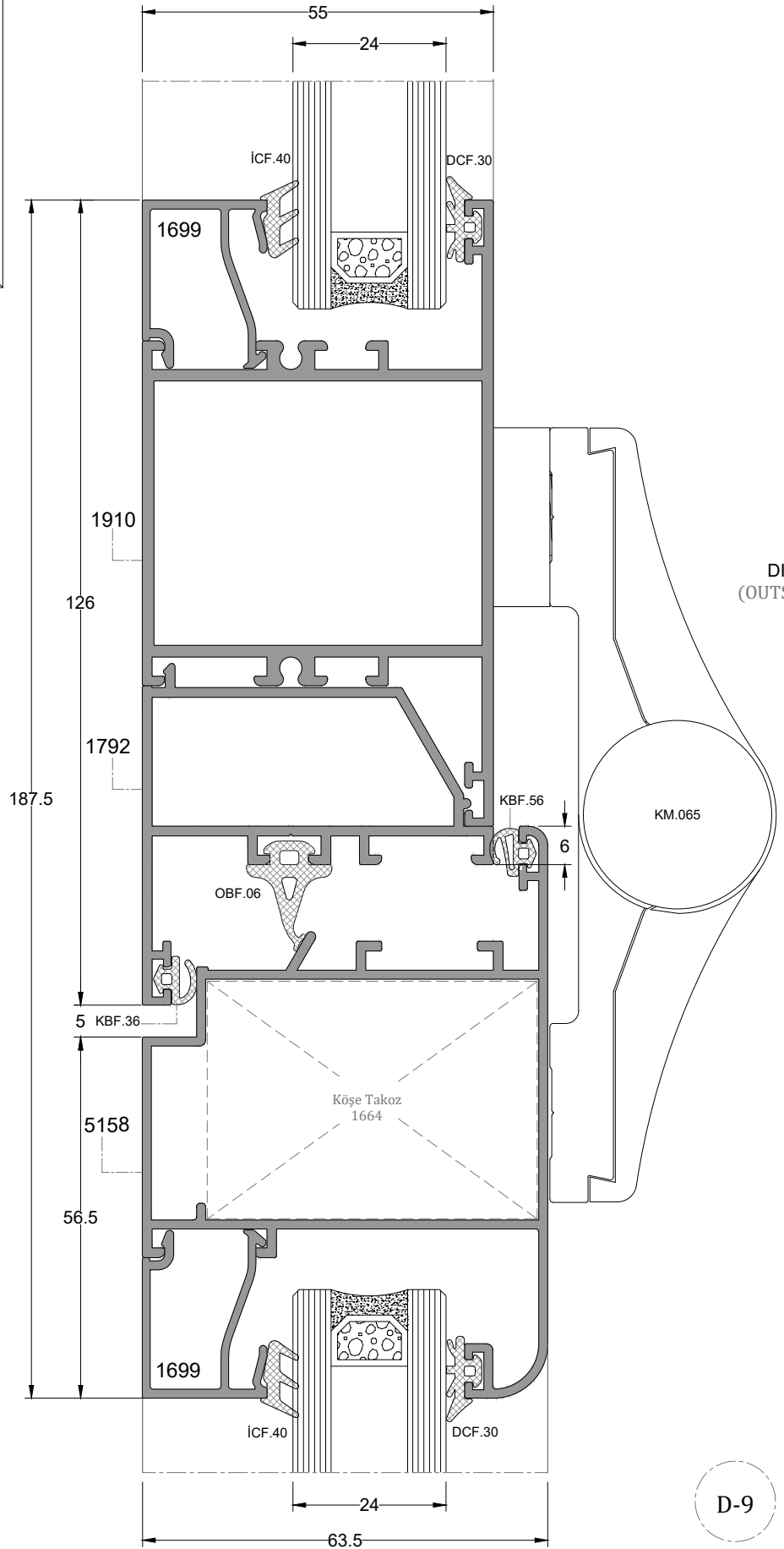
DIŞA AÇILIR BİNLİ KAPI DETAY OUTWARD OPENING OVERLAPPING DOOR DETAIL
