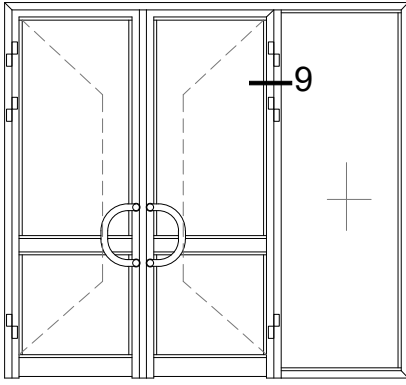
DIŞA AÇILIR BİNLİ KAPI DETAY OUTWARD OPENING OVERLAPPING DOOR DETAIL
